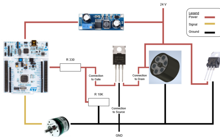
Figure 5.2: Wiring Diagram
